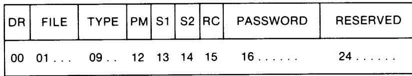
Figure 2-1. XFCB Format
